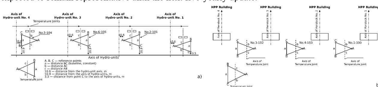
Figure 3 – Layout of the Radon VB-Shch joint gauges with reference points A, B and C: (a) HPP building, el. 446.0 m; (b) water intake [Author's material]
