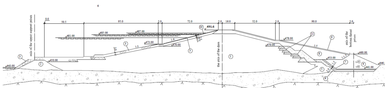
Figure 1 - Typical cross-section of the river-bed dam (zones 1-11 are described in the text) [Author's material]
