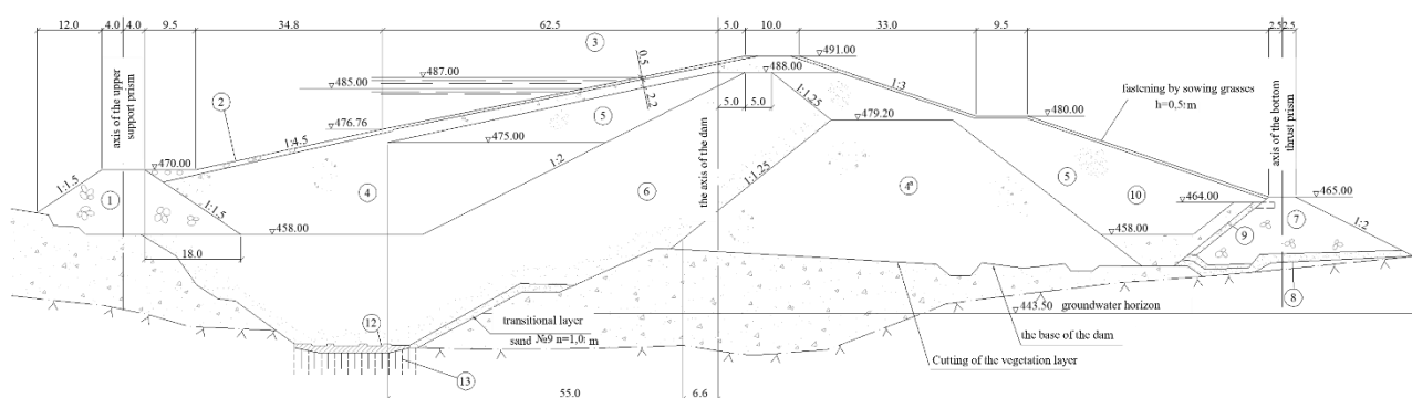
Figure 2 - Typical cross-section of the ravine dam (zones 1-13 are described in the text) [Author's material]
