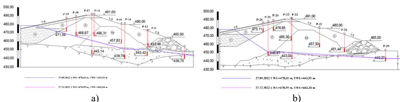
Figure 6 - Phreatic curves in the ravine dam: (a) Section 3 (PK 1+89.5); (b) Section 4 (PK 2+39.5) [Author's material]
