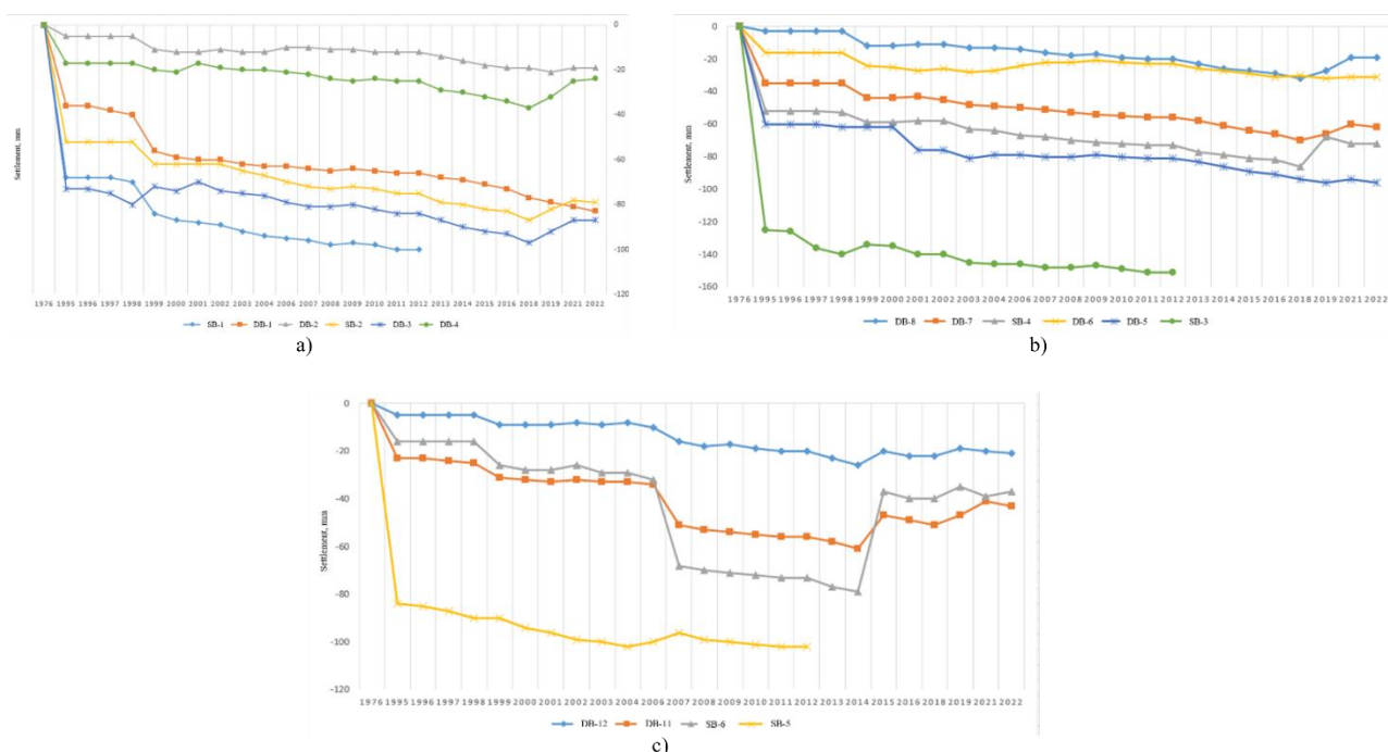
Figure 7 - Settlement of the river-bed dam benchmarks: (a) Section 1; (b) Section 2; (c) Section 3. The time axis is not to scale for 1976–1995 [Author's material]
