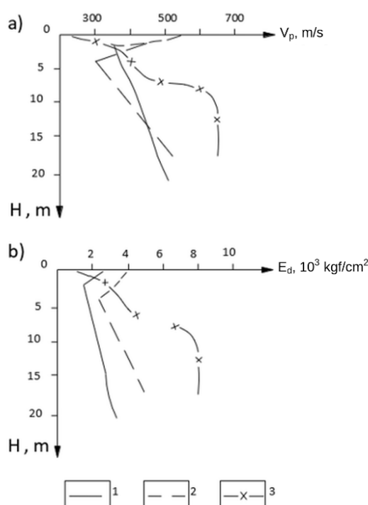
Figure 8 - Depth profiles at the river-bed dam: (a) V_p ; (b) E_d [Author's material]
