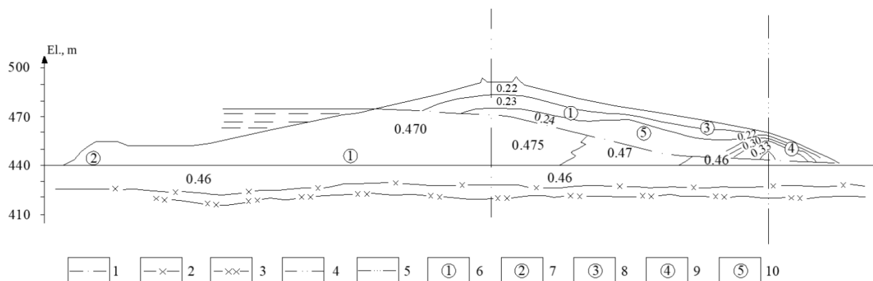
Figure 10 - Distribution of v across the river-bed dam [Author's material]
