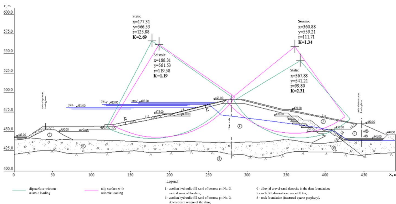
Figure 13 – Critical slip surfaces of the river-bed dam at seismic intensity 9 [Author's material]
