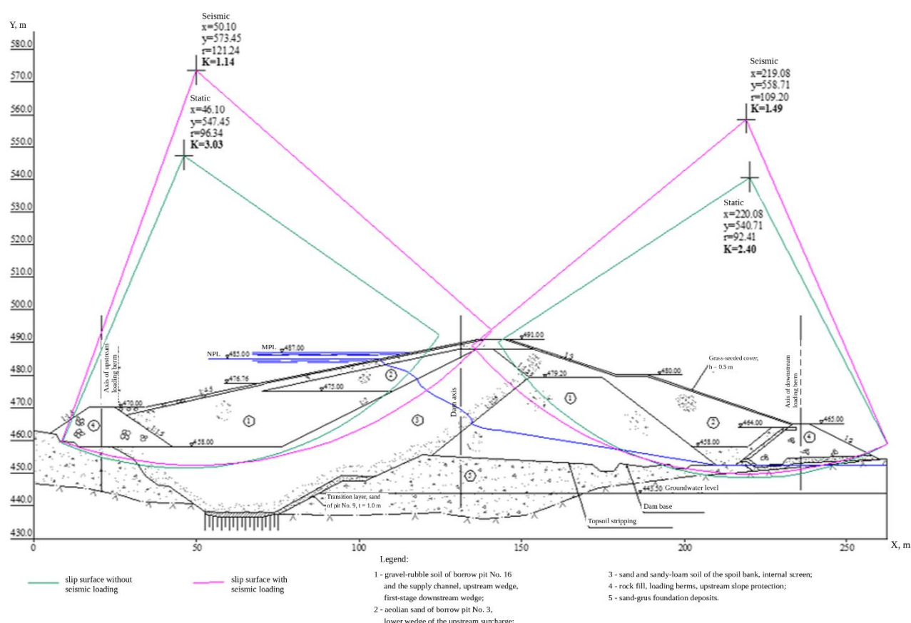
Figure 12 – Slope stability of the ravine dam at seismic intensity 9 [Author's material]
