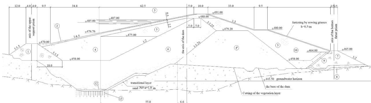
Figure 2 - Typical cross-section of the ravine dam (zones 1-13 are described in the text) [Author's material]
