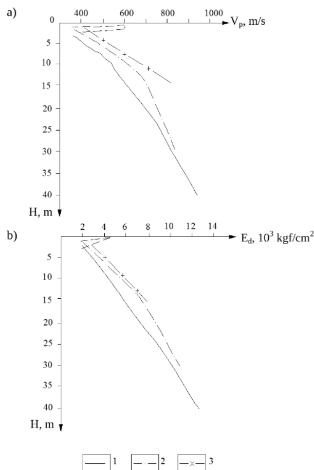
Figure 9 - Depth profiles at the ravine dam: (a) V_p ; (b) E_d [Author's material]
