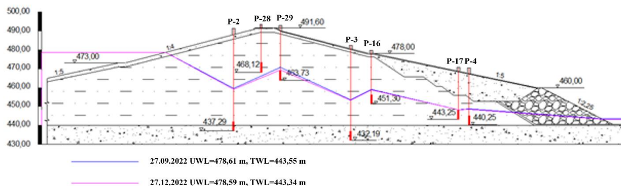
Figure 4 - Phreatic curves in Section 2 (PK 2+50) of the river-bed dam [Author's material]
