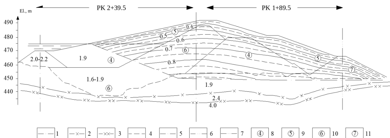
Figure 11 - Distribution of V_p across the ravine dam [Author's material]
