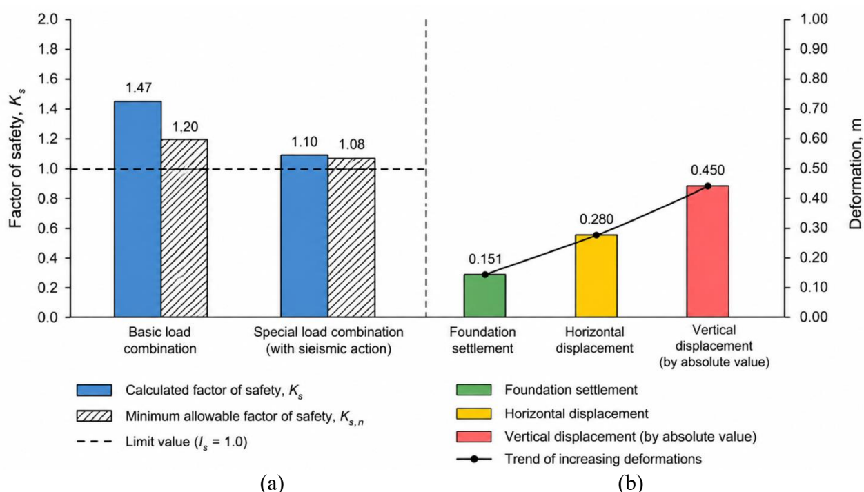
Figure 5 – Integrated assessment of the numerical modelling results for the railway embankment: (a) comparison of the calculated and minimum permissible factors of safety under the basic and special load combinations; (b) maximum calculated deformations after 300 days of consolidation [Authors' material]
