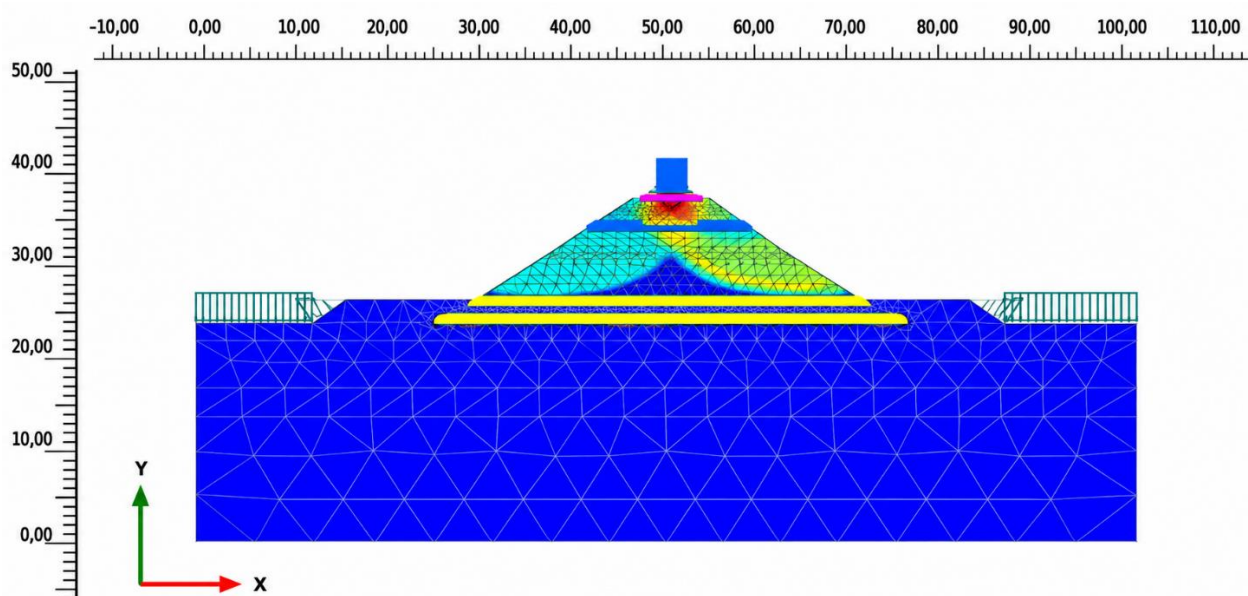
Figure 2 – Calculated position of the potential failure surface of the railway embankment under the basic load combination [Authors' material]
