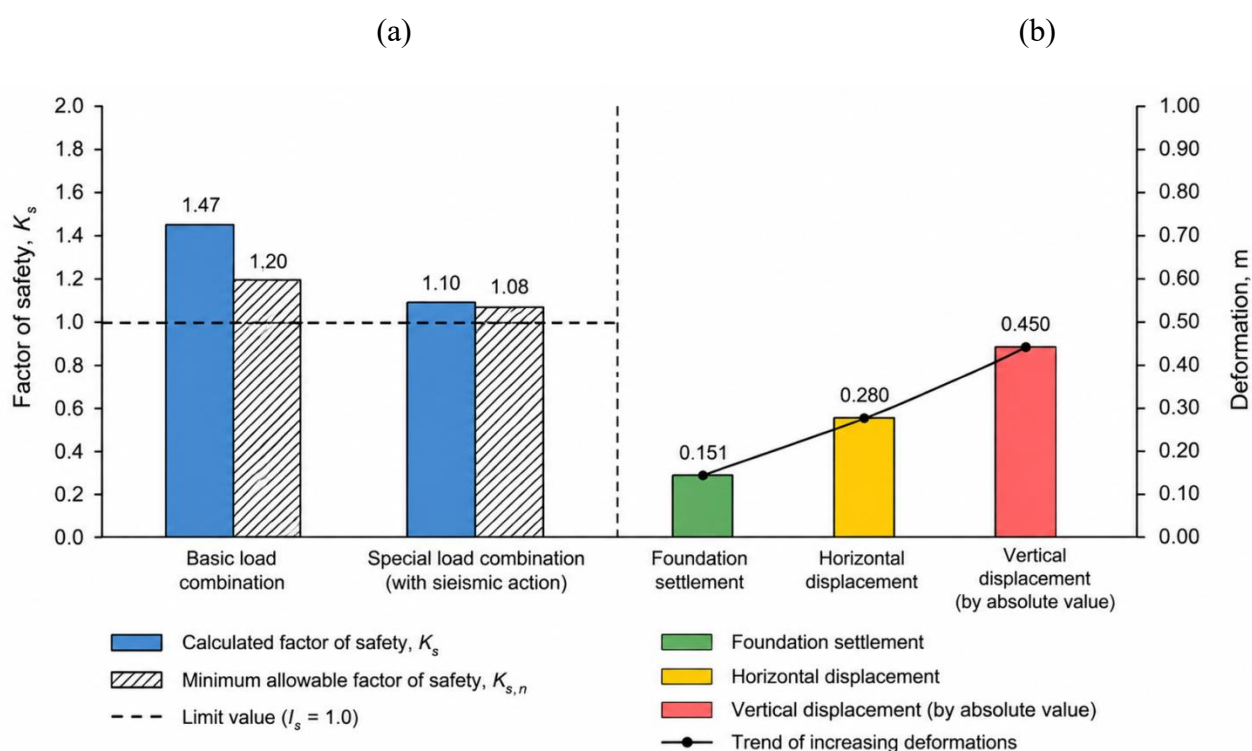
Figure 5 – Integrated assessment of the numerical modelling results for the railway embankment: (a) comparison of the calculated and minimum permissible factors of safety under the basic and special load combinations; (b) maximum calculated deformations after 300 days of consolidation [Authors' material]
