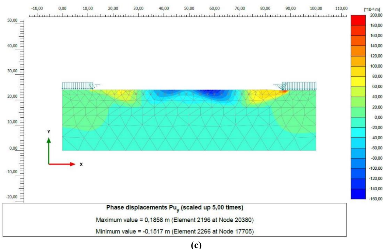
Figure 4 – Deformation behaviour of the railway embankment after 300 days of consolidation: (a) foundation settlement; (b) horizontal displacements; (c) vertical displacements [Authors' material]
