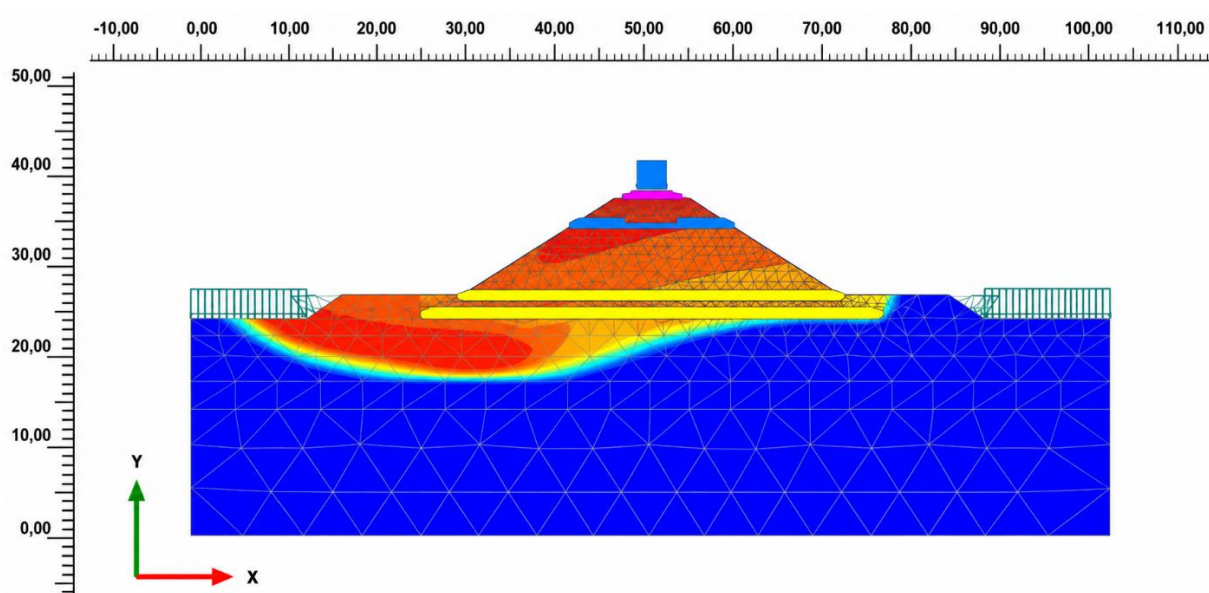
Figure 3 – Calculated position of the potential failure surface of the railway embankment under the special load combination incorporating seismic action [Authors' material]
