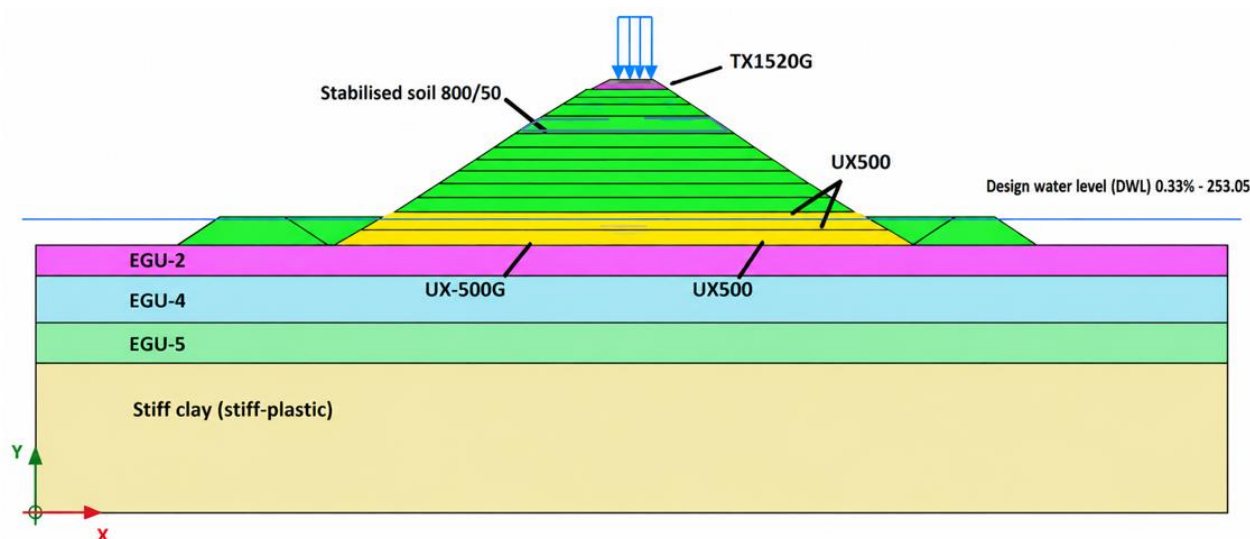
Figure 1 – Numerical model of the railway embankment with the gravel layer positioned above the design high-water level and the foundation reinforced with geosynthetic materials [Authors' material]
