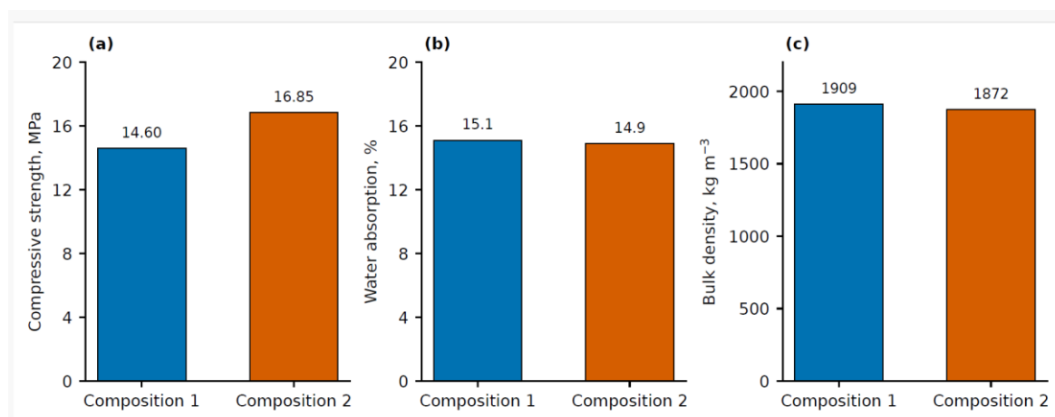
Figure 9 – Comparison of the compressive strength (a), water absorption (b), and bulk density (c) of the fired ceramic specimens [Author's material]
