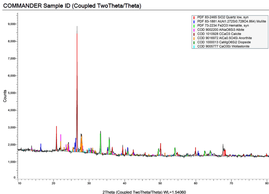
Figure 7 – XRD pattern of fired Composition 1 containing 50.0 wt.% clay and 50.0 wt.% ground ASW; firing temperature: 950 °C [Author's material]
