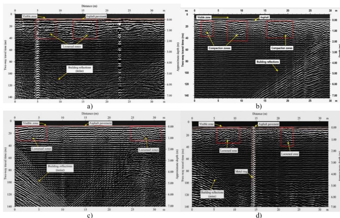
Figure 7 - (a) GPR radargram - Transverse Profile 0010. (b) GPR radargram - Transverse Profiles 0012-0013. (c) GPR radargram - Transverse Profile 0016. (d) GPR radargram - Transverse Profile 0018 [Author's material]
