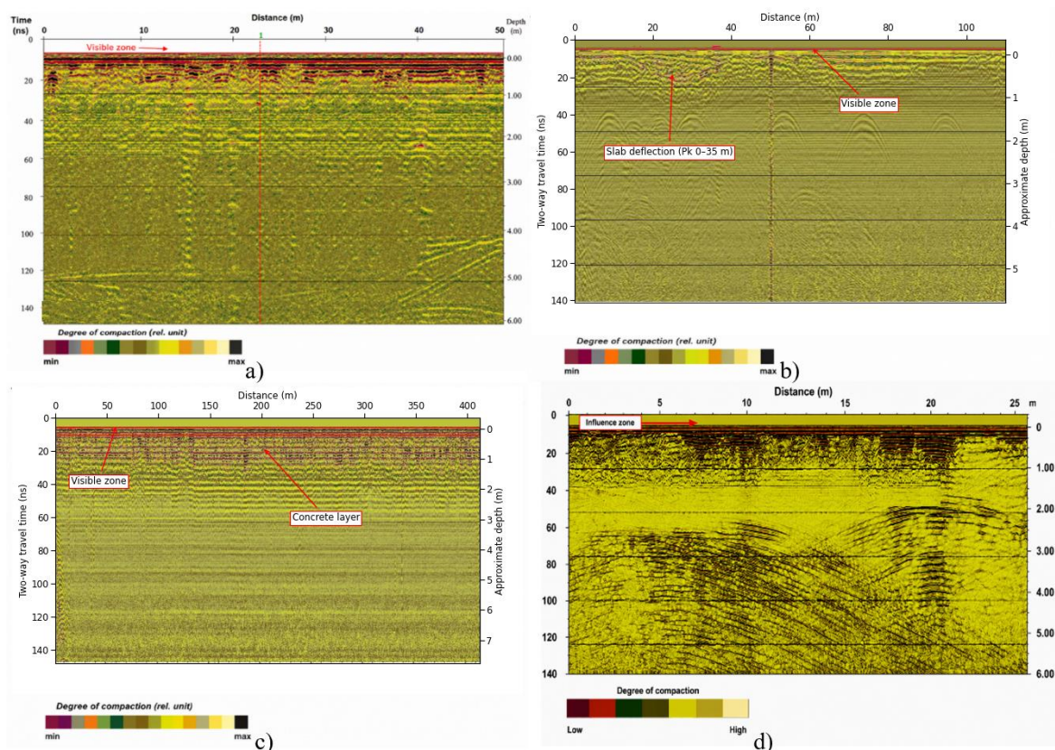
Figure 8 - (a) Interpretation of Radargram No. 19 (Profile 001), tailrace-channel lining, right bank; (b) Interpretation of Radargram No. 21 (Profile 003), tailrace-channel lining, right bank; (c) Interpretation of Radargram No. 23 (Profile 049), river-bed dam, upstream slope; (d) Interpretation of Radargram No. 31 (Profile 019), the ravine dam, upstream slope [Author's material]
