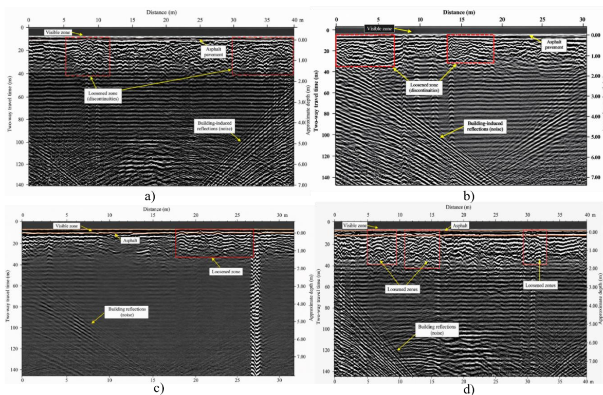
Figure 6 - (a) GPR radargram - Longitudinal Profile 001. (b) GPR radargram - Longitudinal Profile 002. (c) GPR radargram - Longitudinal Profile 004. (d) GPR radargram - Longitudinal Profile 006 [Author's material]
