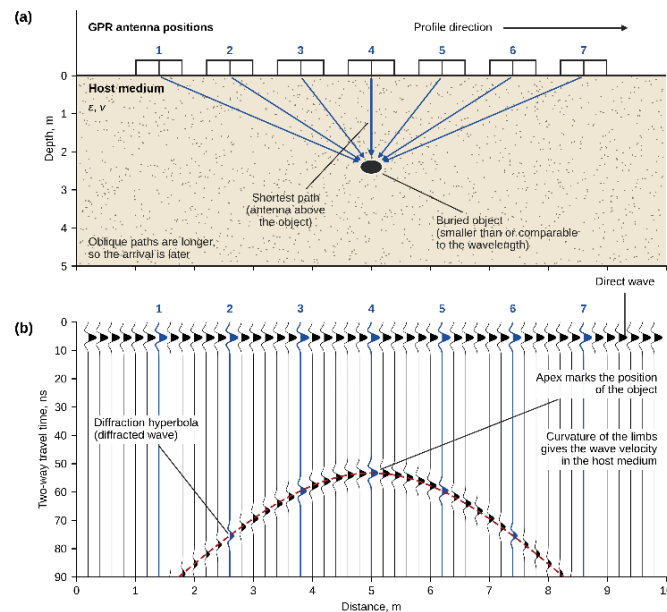
Figure 4 - Formation of a diffraction hyperbola from a discrete buried object as the antenna moves along the profile: (a) ray paths from successive antenna positions (1-7) to the object; (b) synthetic traces (150 MHz wavelet) at the same positions (highlighted in blue) showing the direct wave and the diffracted wave, whose arrival times form a hyperbola. Schematic with illustrative values [Author's material]
