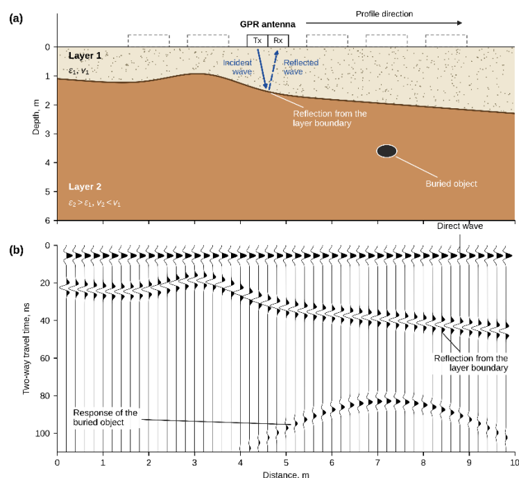
Figure 3 - Basic operating principle of ground-penetrating radar: (a) geological section with the GPR antenna, two layers of different permittivity ( \epsilon_2 > \epsilon_1 ) and a buried object; (b) synthetic traces (150 MHz wavelet) showing the direct wave, the reflection from the layer boundary and the diffraction hyperbola from the object. Schematic with illustrative values [Author's material]
