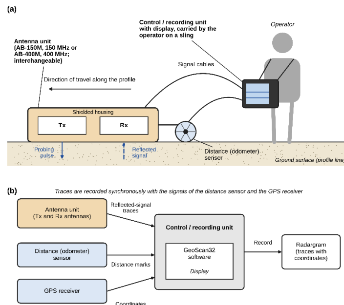
Figure 5 - OKO-3 ground-penetrating radar: (a) field configuration, in which the shielded antenna unit (transmitting, Tx, and receiving, Rx, antennas) is moved along the profile, the distance sensor triggers the recording, and the control/recording unit is carried by the operator on a sling; (b) data-acquisition scheme. [Author's material]
