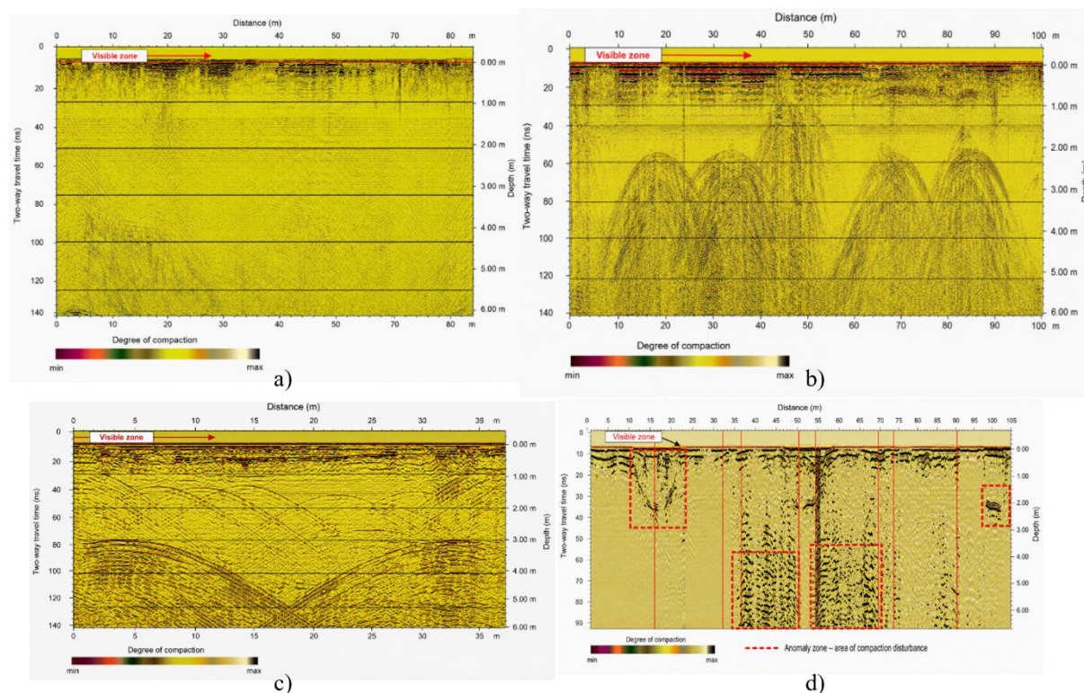
Figure 9 - (a) Interpretation of Radargram No. 46 (Profile 034), 220 kV switchyard platform; (b) Interpretation of Radargram No. 52 (Profile 040), 220 kV switchyard platform; (c) Interpretation of Radargram No. 54 (Profile 043), 220 kV switchyard platform; (d) Interpretation of Radargram No. 60 (Profile 060), stop-log storage area, along the line of observed ground disturbance [Author's material]
