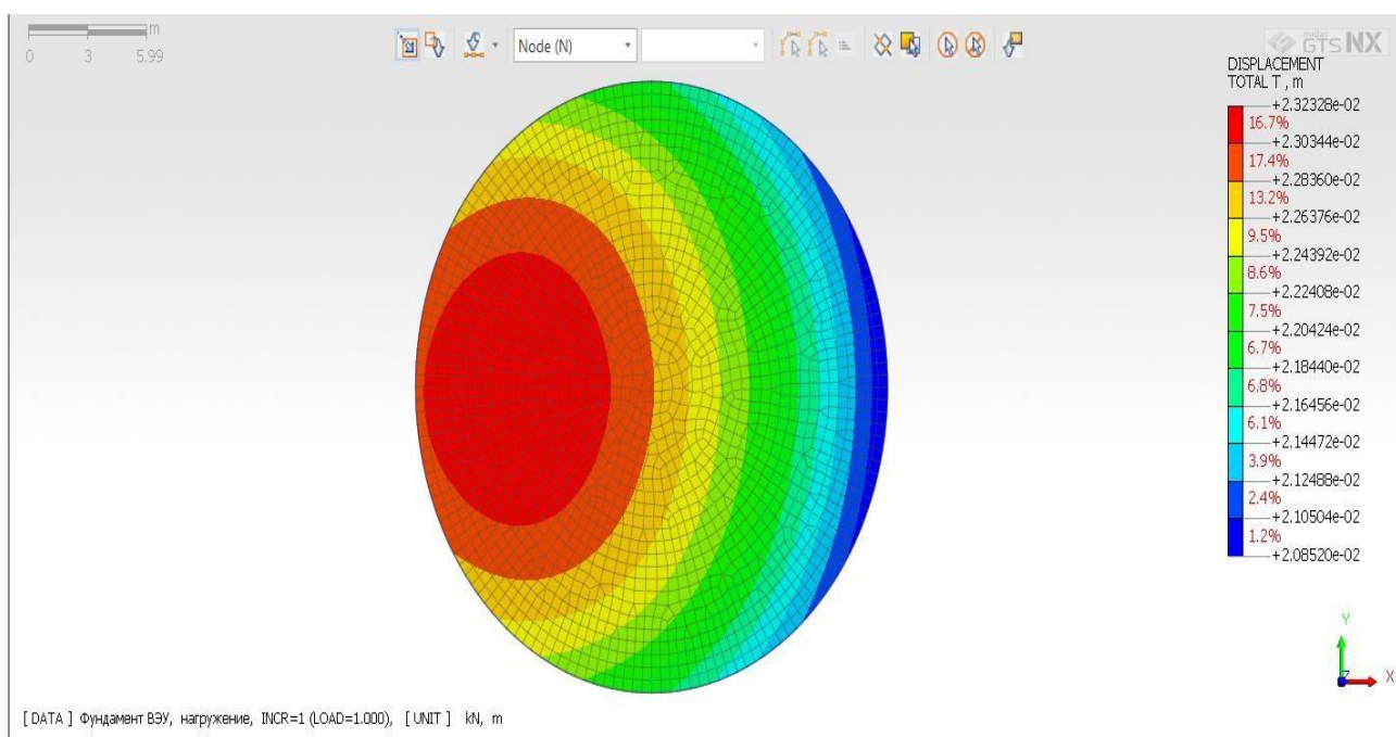
Figure 4 - Total Foundation Deformations (max. 2.32 cm; min. 2.08 cm).
