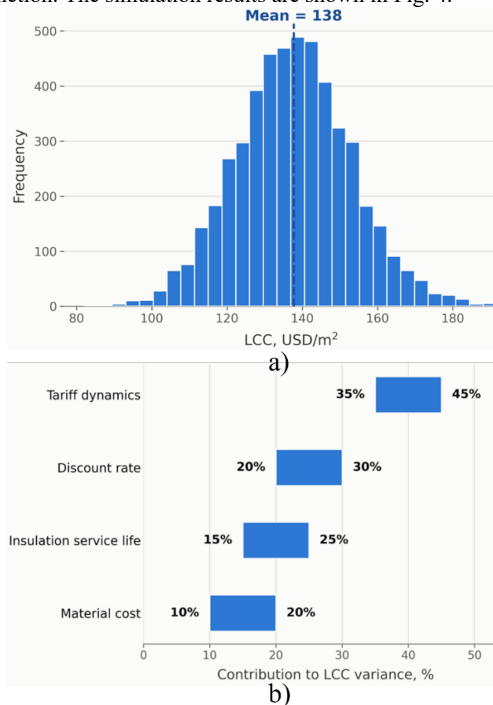
Figure 4 – LCC distribution from Monte Carlo simulation and the contribution of factors to its variance a) Monte Carlo LCC distribution ( N = 5000 ) b) Sensitivity: factor contribution to LCC variance [Authors' material]
