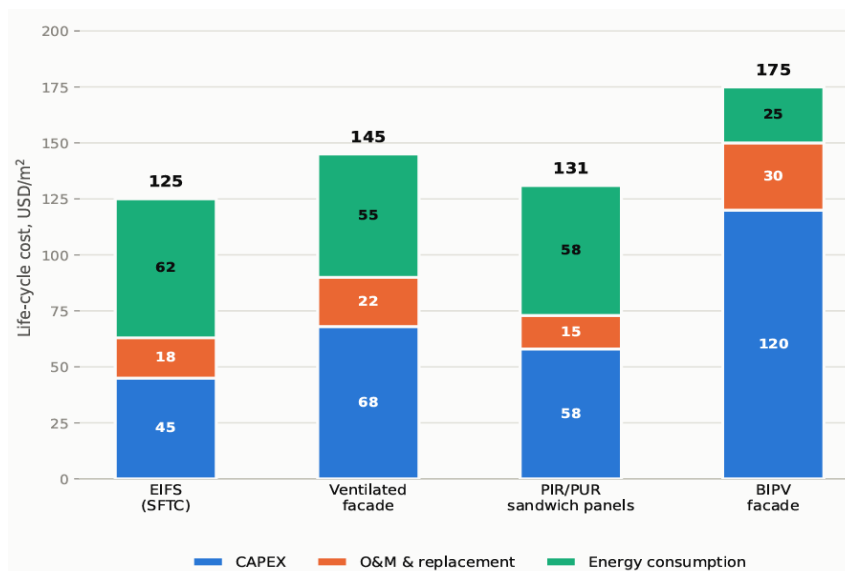
Figure 3 – Life-cycle cost (LCC) structure by facade system (illustrative calculation) [Authors' material]
