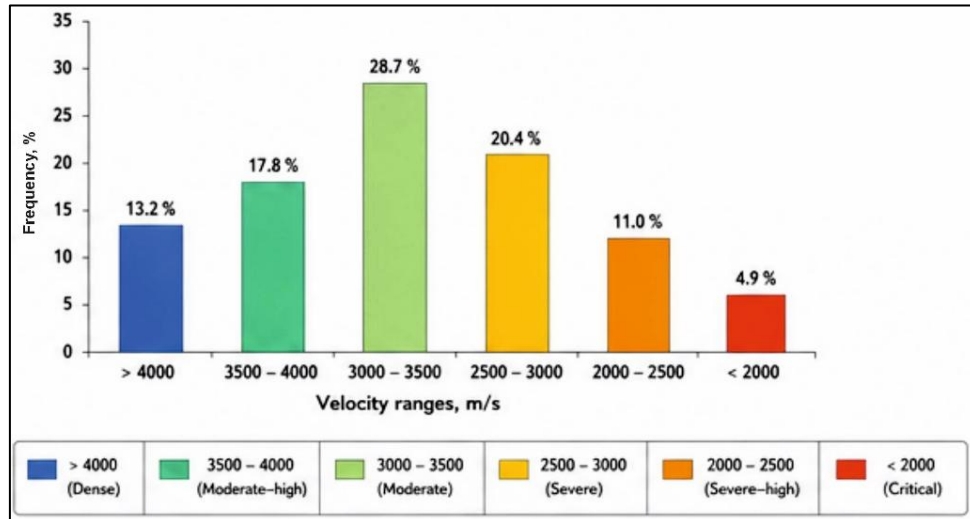
Figure 13 - Statistical distribution of ultrasonic wave velocities (authors' material)
