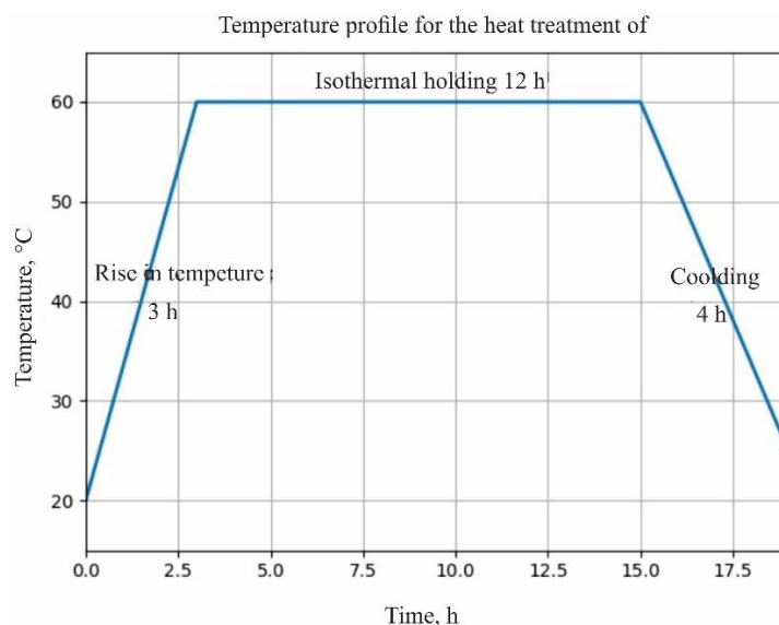
Figure 2 – Stages of heat treatment of three-layer wall panels (author's material)
