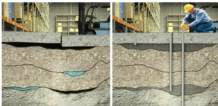
Figure 5 - Soil reinforcement by injection method (catalogue SK Stroiz, 2024)
