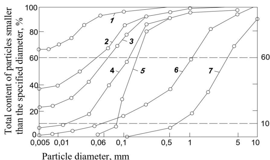
Figure 1 - Curves of the granulometric composition of sandy-silty-clay soils:
