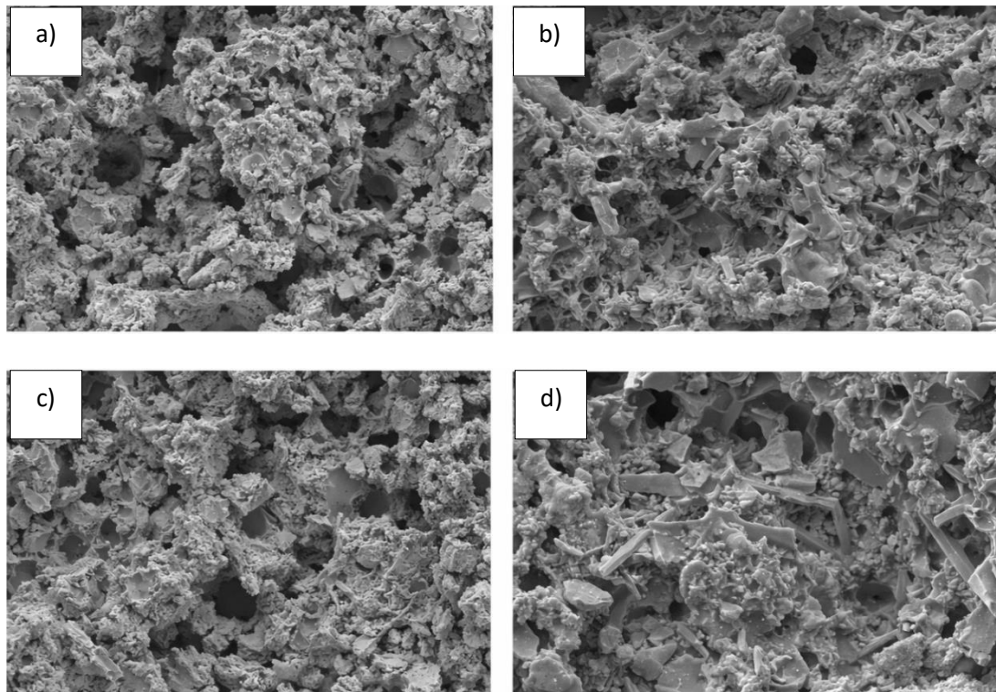
Figure 4 - Microstructure of clay-ash samples after firing at 1100 and 1400 °C (SEM): a) 90:10, 1100 °C; b) 90:10, 1400 °C; c) 50:50, 1100 °C; d) 50:50, 1400 °C (author's materials)
