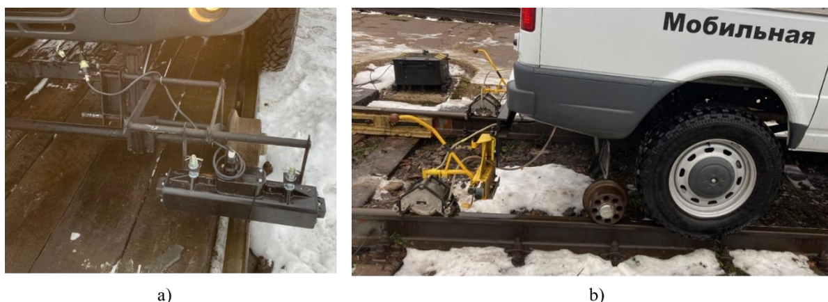
Figure 2 – MDL flaw detection equipment (a) Front view of the meter; (b) Side view of the meter [Authors' material]
