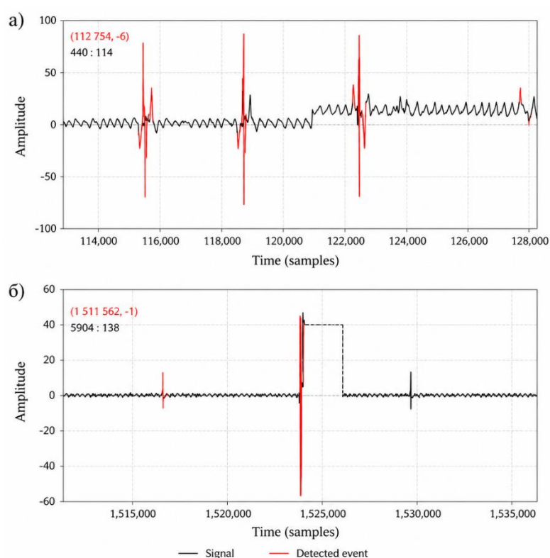
Figure 4 – Flaw patterns, zero-line offset signals: a) is the case of a relatively small displacement of the zero line; b) the case of a critical offset incompatible with the normal functioning of the channel [Authors' material]
