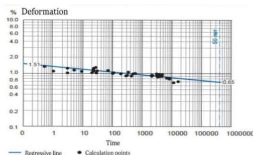
Figure 9 – Deformation under pressure chart (Flowtime piping systems. 2025)
