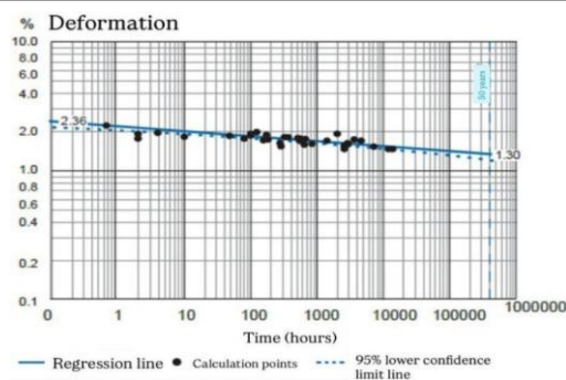
Figure 11 – Diametral deformation chart under long-term loading on a pipe in water (Flowtime piping systems.2025)
