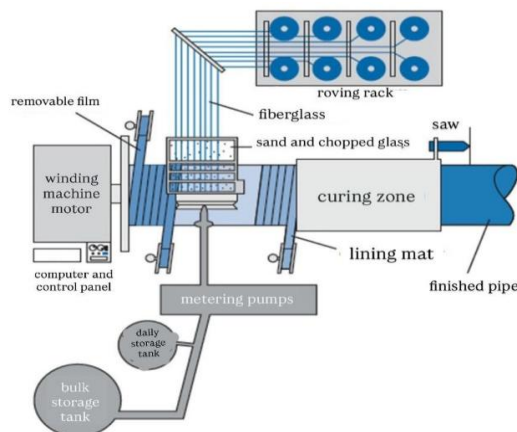
Figure 7 – Fiberglass-reinforced plastic pipe manufacturing scheme (Flowtime piping systems, 2025)
