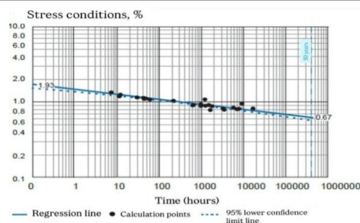
Figure 8 – Corrosion resistance chart under stressed conditions (Flowtime piping systems.2025)
