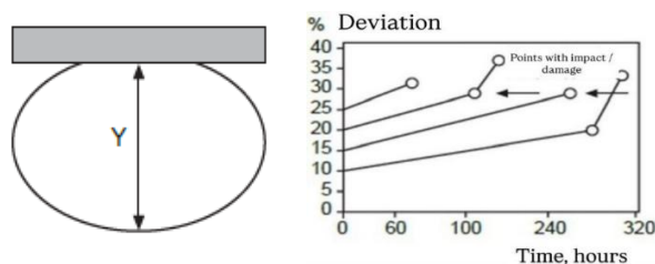
Figure 10 – Effect of long-term loading in water on diametral deformation (Flowtime piping systems.2025)
