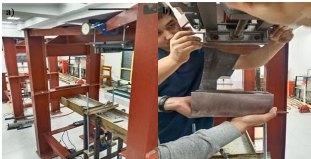
Figure 2 – Tensile testing machine of the geotechnical laboratory (a) and the process of conducting a tensile test of a geogrid sample (b) (author's materials)
