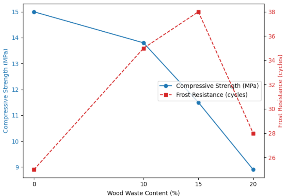
Figure 6 – Effect of wood waste content on compressive strength and frost resistance of ceramic materials (author's material)
