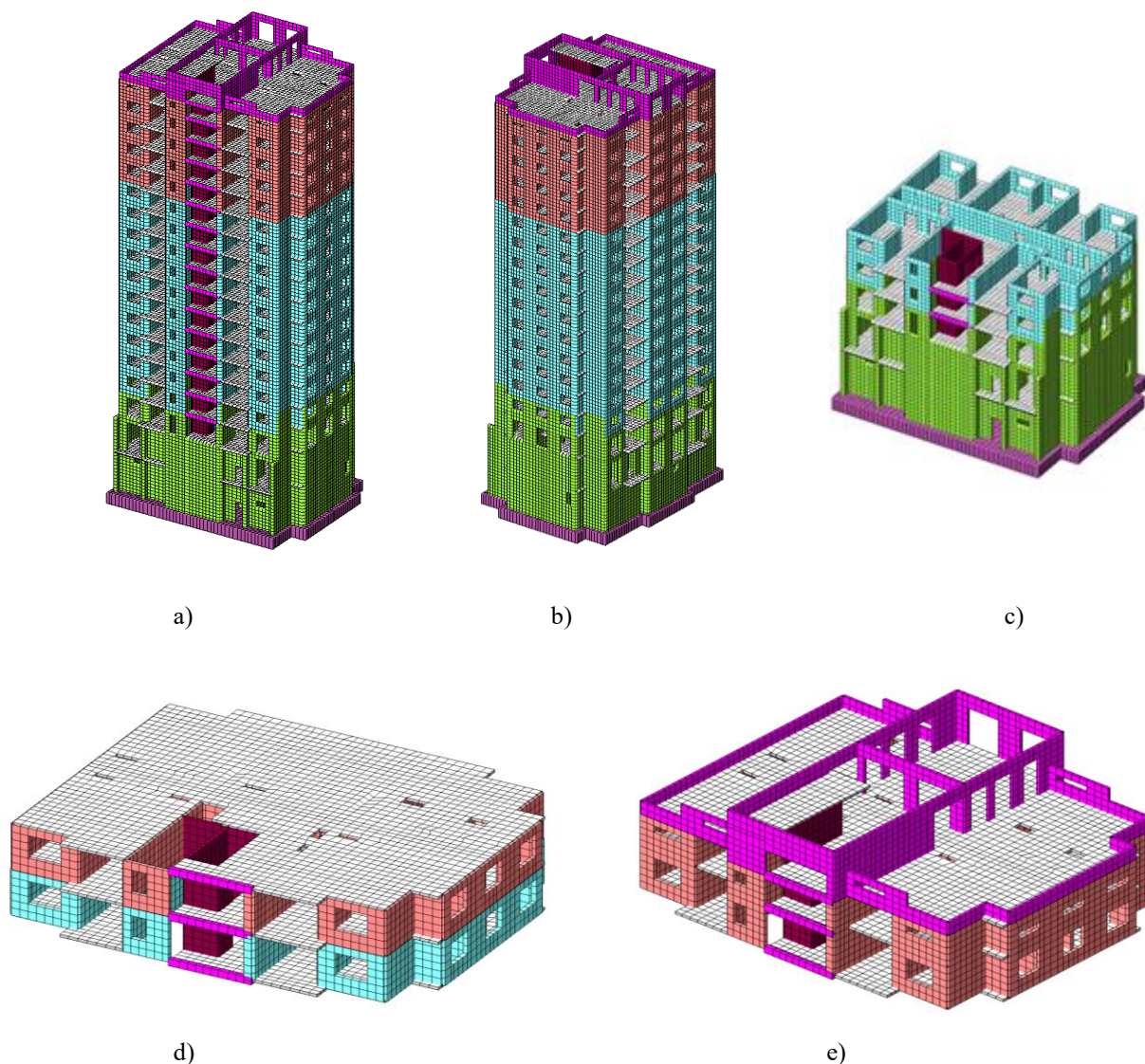
Figure 1 – General Views of the Computational Model (a, b, c, d, e) (author's material)
