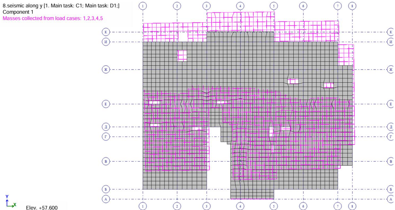
Figure 6 - Displacement mosaic along the Y -axis (author's material)
