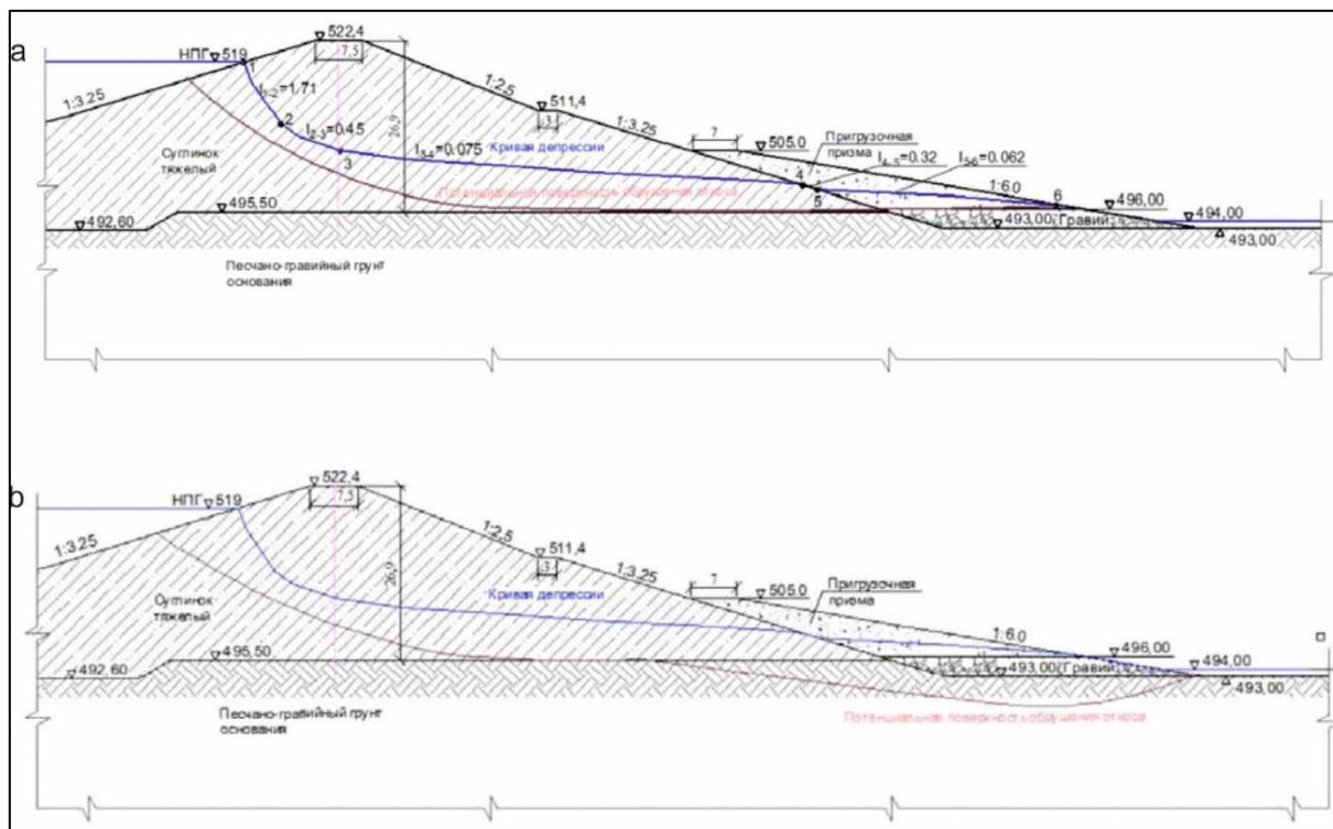
Figure 7 – Calculation Schemes: a – PK 5+00, Load Case 1, Seismic Intensity – 7 points, Safety Factor ( k ) = 1.227; b – PK 5+00, Load Case 2, Seismic Intensity – 8 points, Safety Factor ( k ) = 1.035
